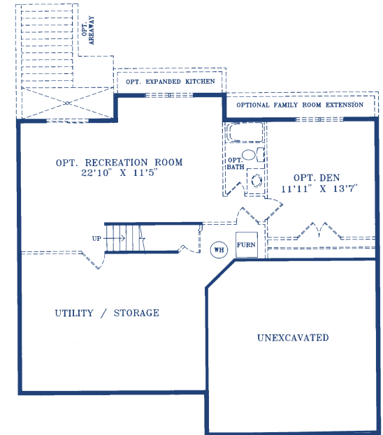
Lower Level Floor Plan
