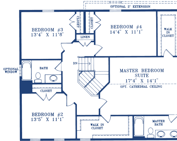
Alternate Upper Level Floor Plan
