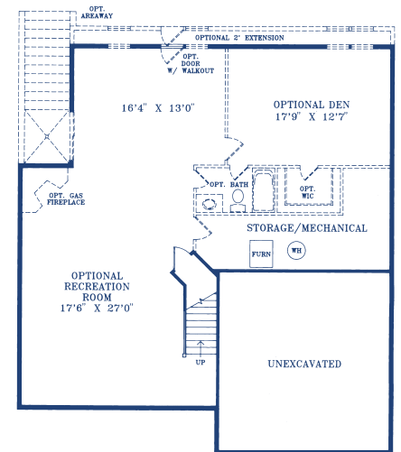
Lower Level Floor Plan
