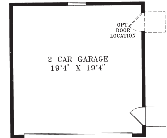
GARAGE FLOOR PLAN
