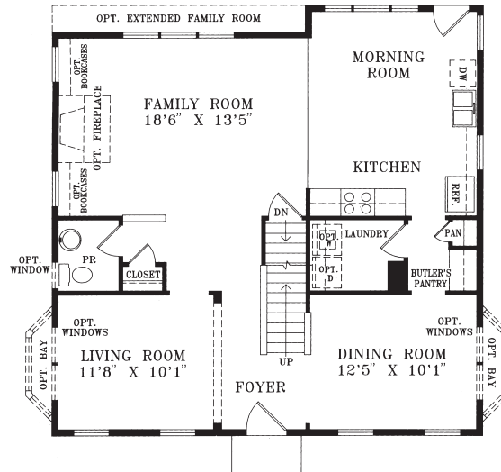
FIRST LEVEL FLOOR PLAN
