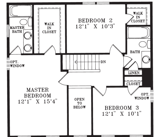
SECOND LEVEL FLOOR PLAN
