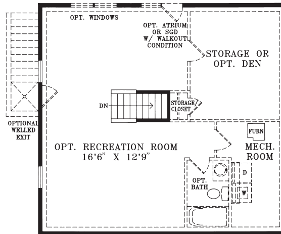
LOWER LEVEL FLOOR PLAN
