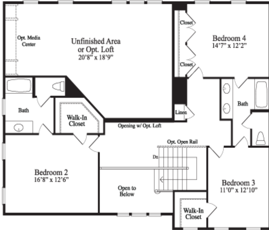
Upper Level Floor Plan with Opt. Loft
