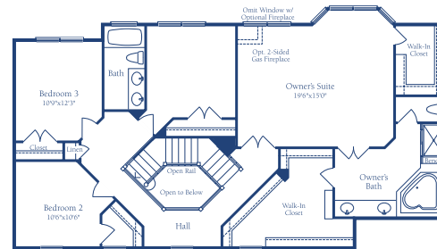
Alternate Second Floor Plan
